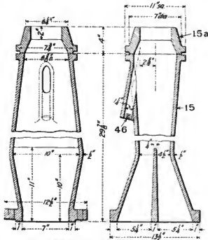
Figs. 370-372. Exhaust Pipe and Nozzle. Southern Pacific.
